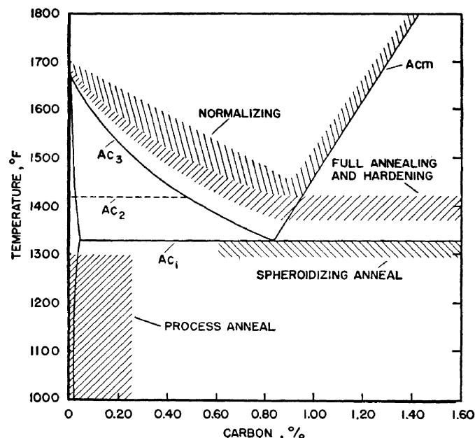
FIGURE 11. Recommended temperature ranges for heat treating plain carbon steels.
