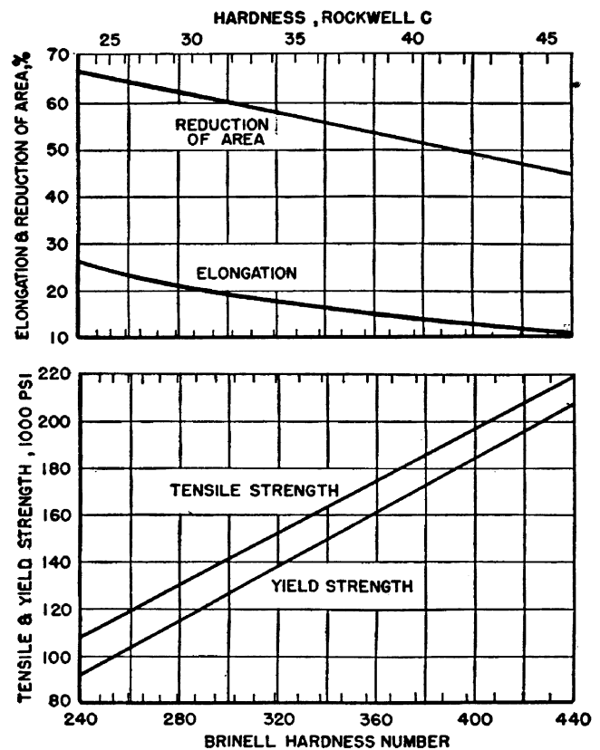
FIGURE 27. Tensile strength, yield strength, elongation, and reduction of area as a function of hardness in structural steels.
