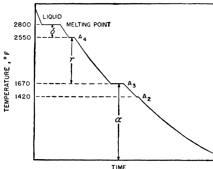
FIGURE 1. Idealized cooling curve for pure iron.
