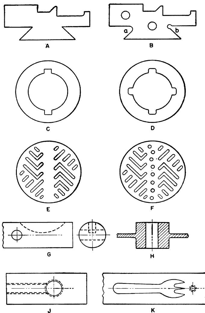
FIGURE 26. Examples of good and bad designs from standpoint of hardening by heat treatment (Palmer and Luerssen, Tool steel simplified , p. 392, 1948).
