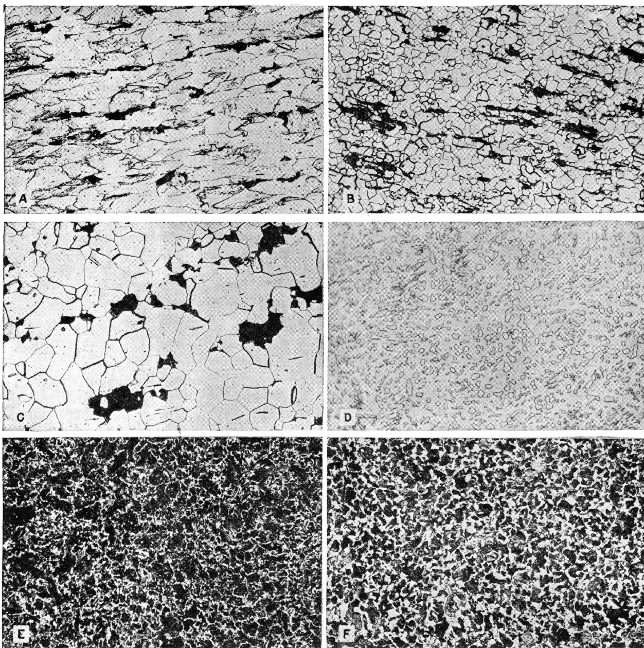
FIGURE 12. Representative microstructures of carbon steels.
