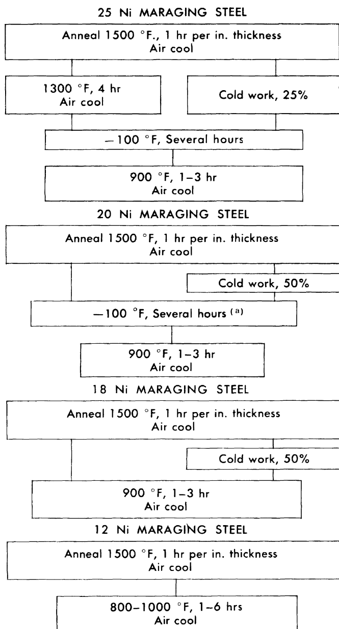
FIGURE 29. Heat treating ranges for Ni maraging steels
