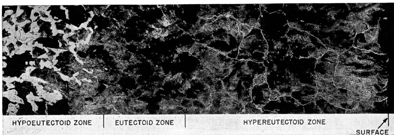
FIGURE 18. Structure of a carburized steel.
