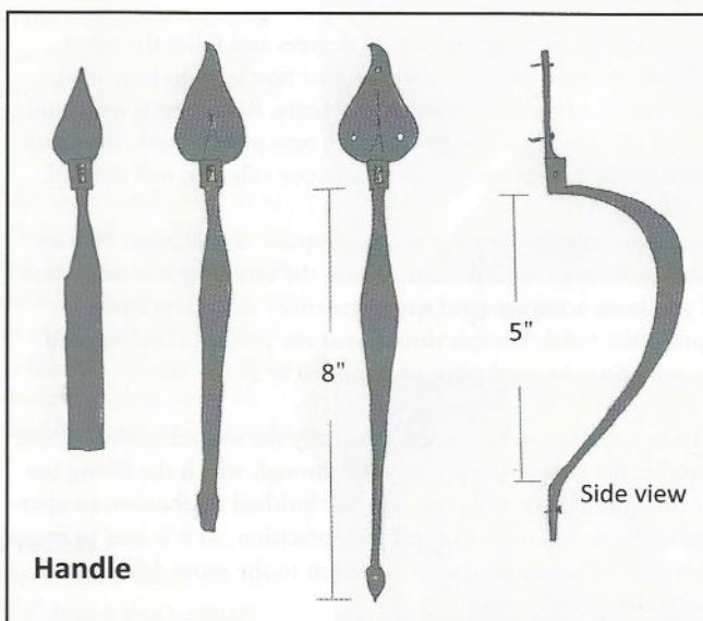
Image #7: Forging and bending the handle.
