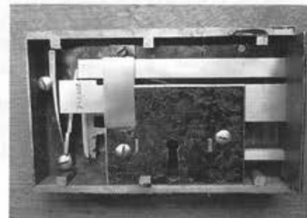
Right: Three-bolt lock works. Reproduction. Forged and filed mild steel, wrought iron, high carbon steel. Painted. 4-1/2" x 7"
