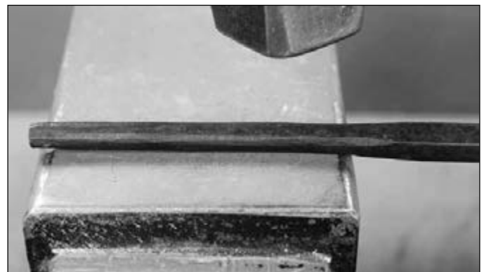
Dress the forging and take to octagon and then on to round
