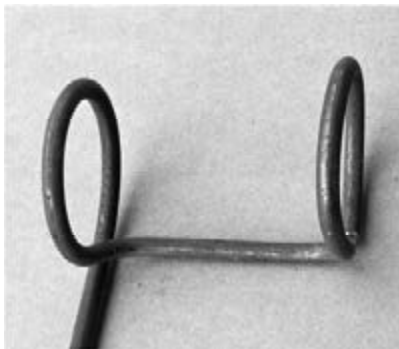
The finished second hoop
