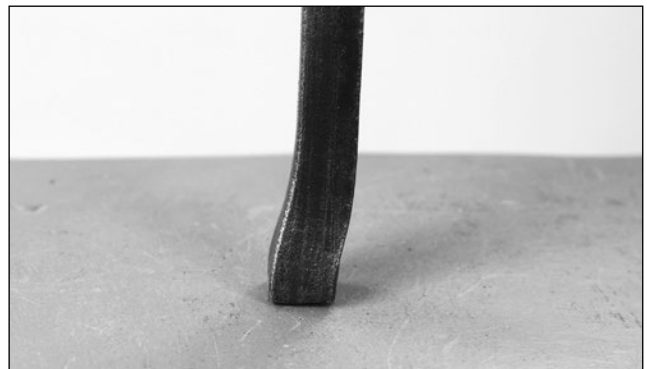
Nothing good ever follows continuing to forge a bent or twisted bar! Take the time to straighten the upset end
